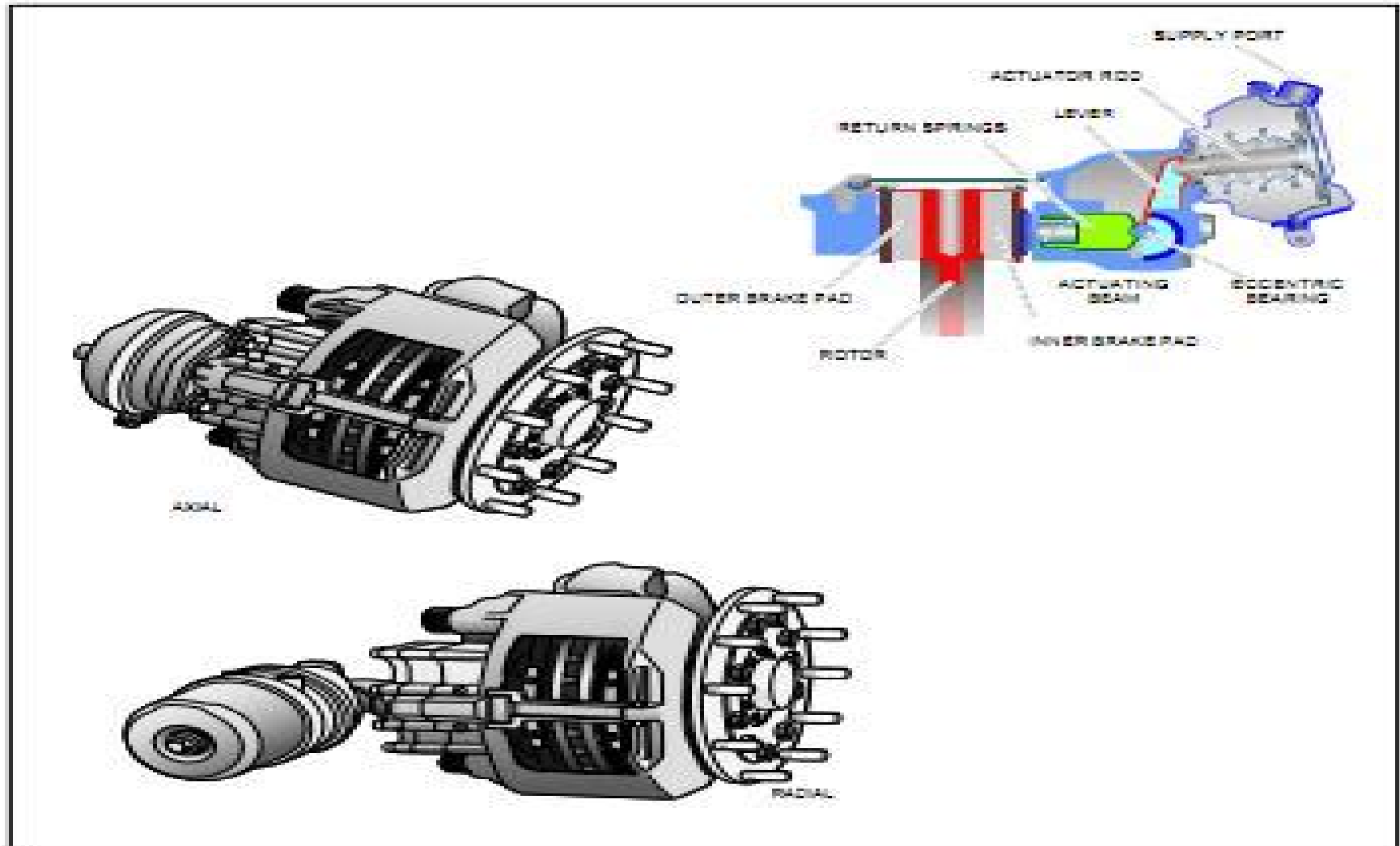
FIGURE 1 - BENDIX AIR DISC BRAKE
