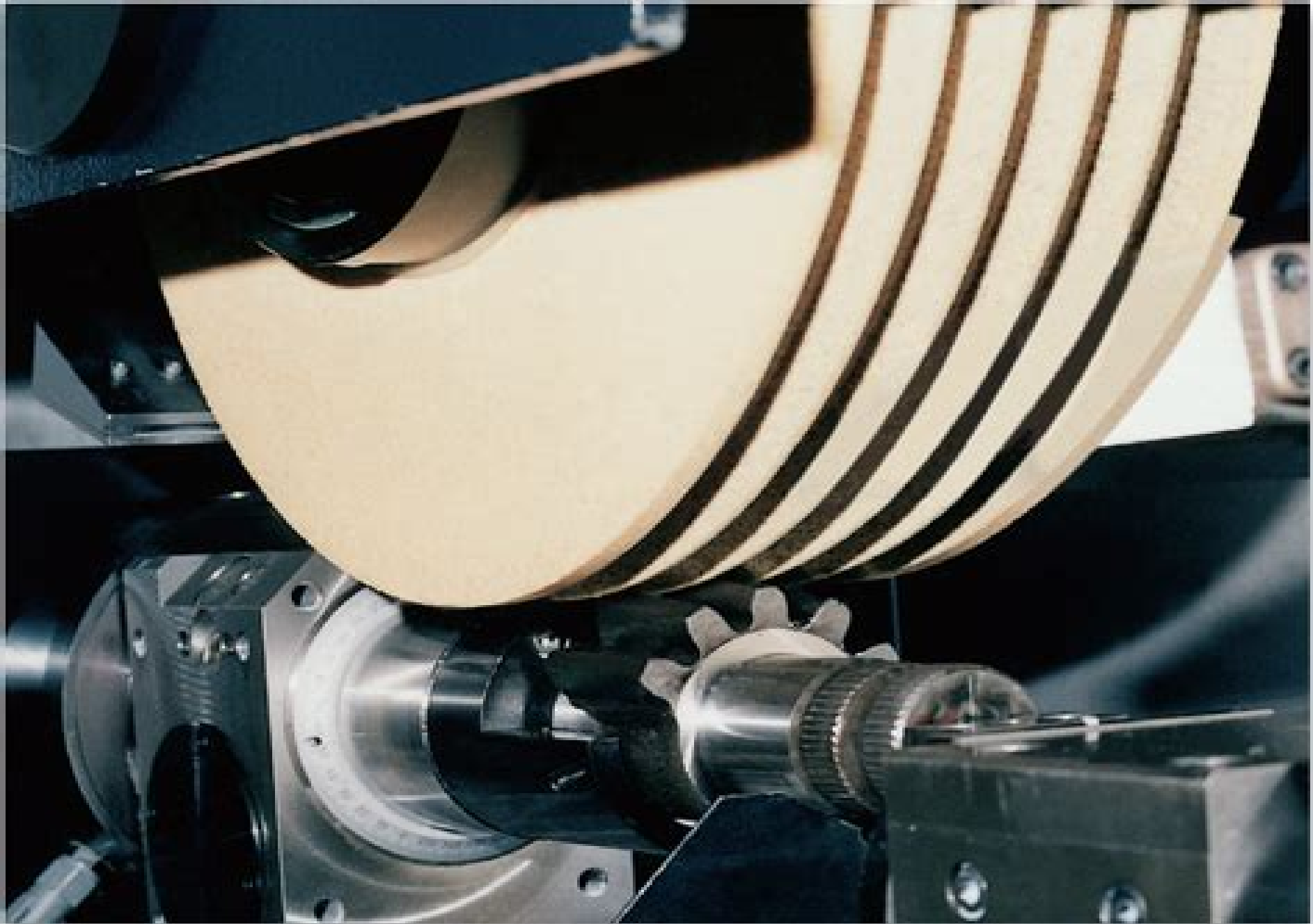
Creep-feed grinding can be considered abrasive or small-chip machining, capable of replacing milling or broaching in the machining of slots and complex forms.
