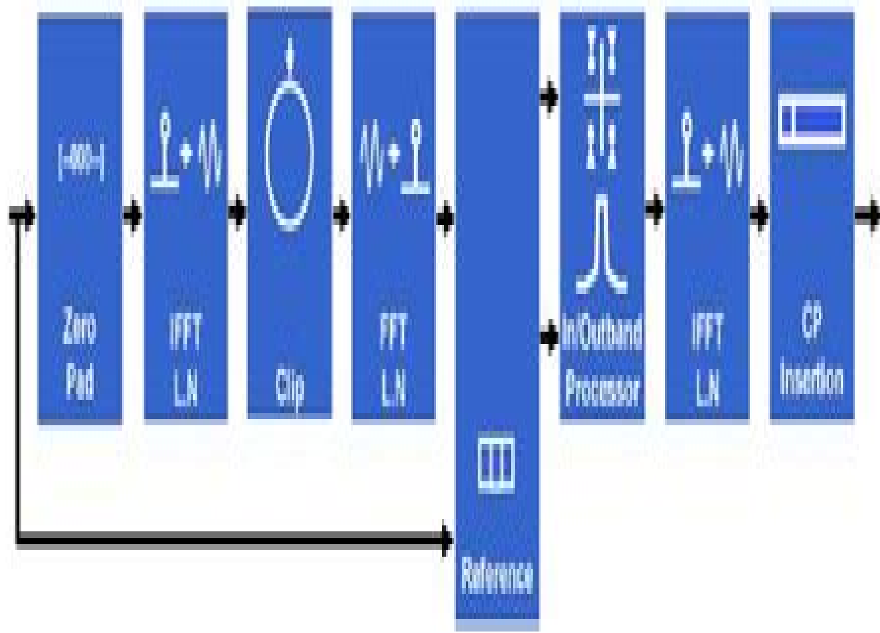
Figure 1. CFH Algorithm Block Diagram of the Necessary Processing
