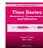
Time Series
