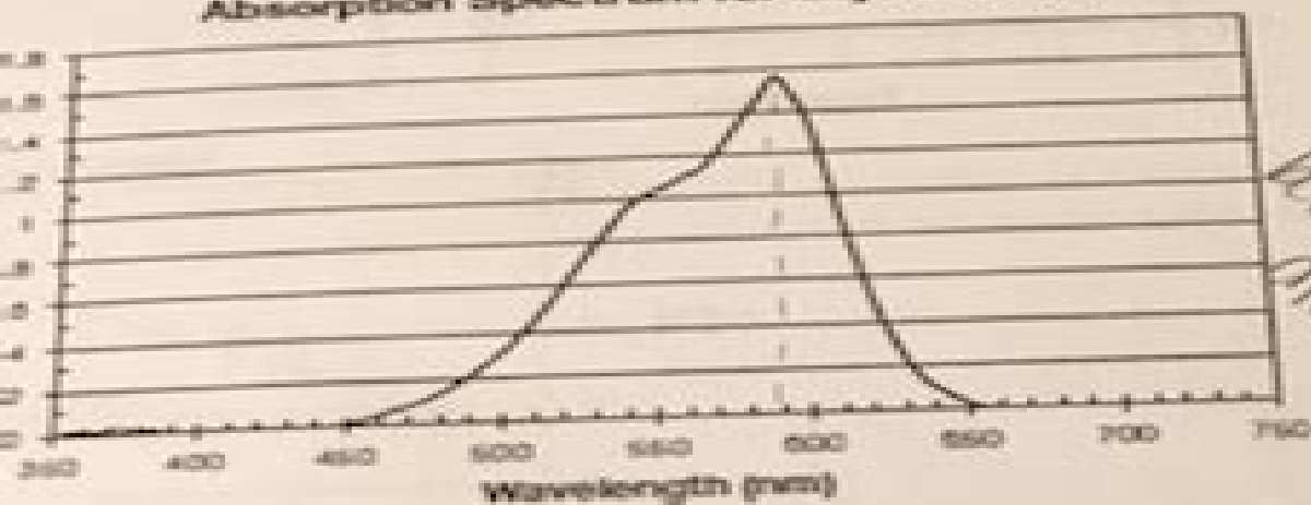
Absorption Spectrum for Crystal Violet
