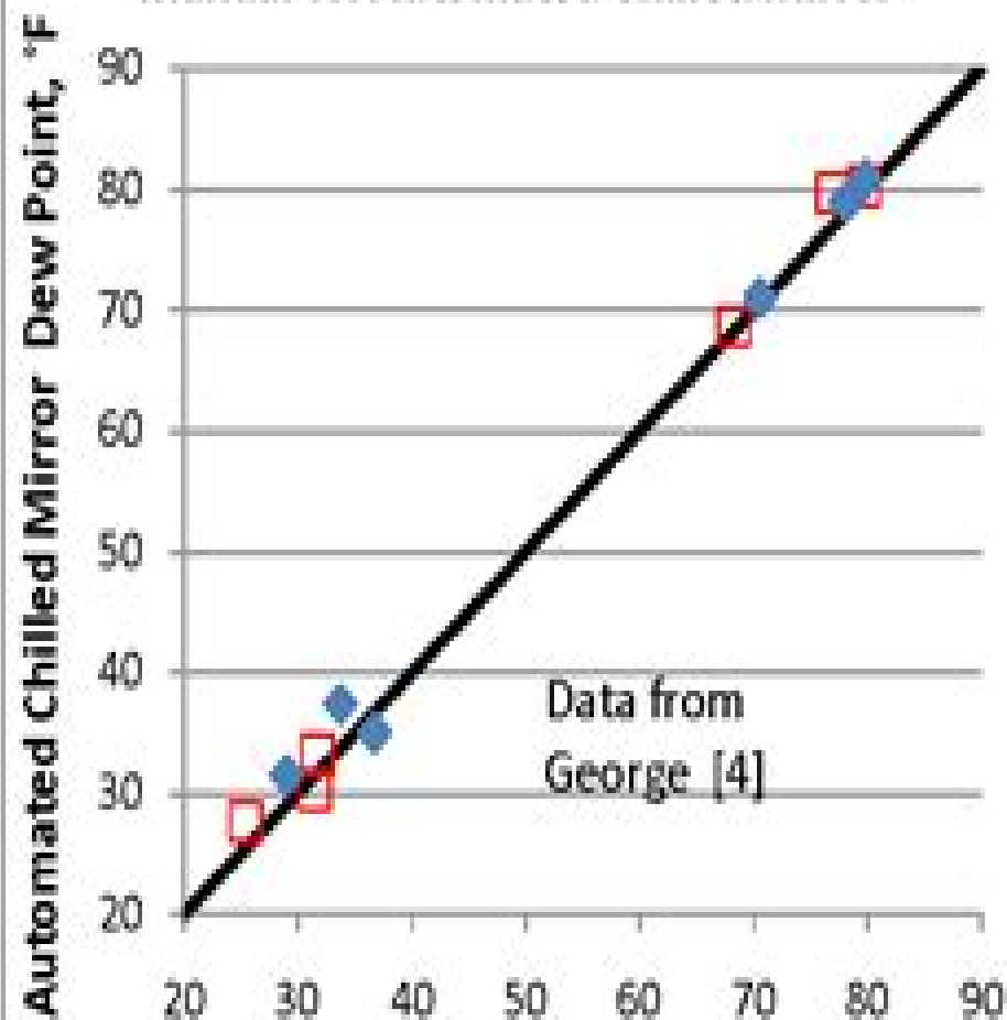
Figure 4 GPA RR-196 Natural Gas Dew Point Manual vs. Automated Chilled Mirror
