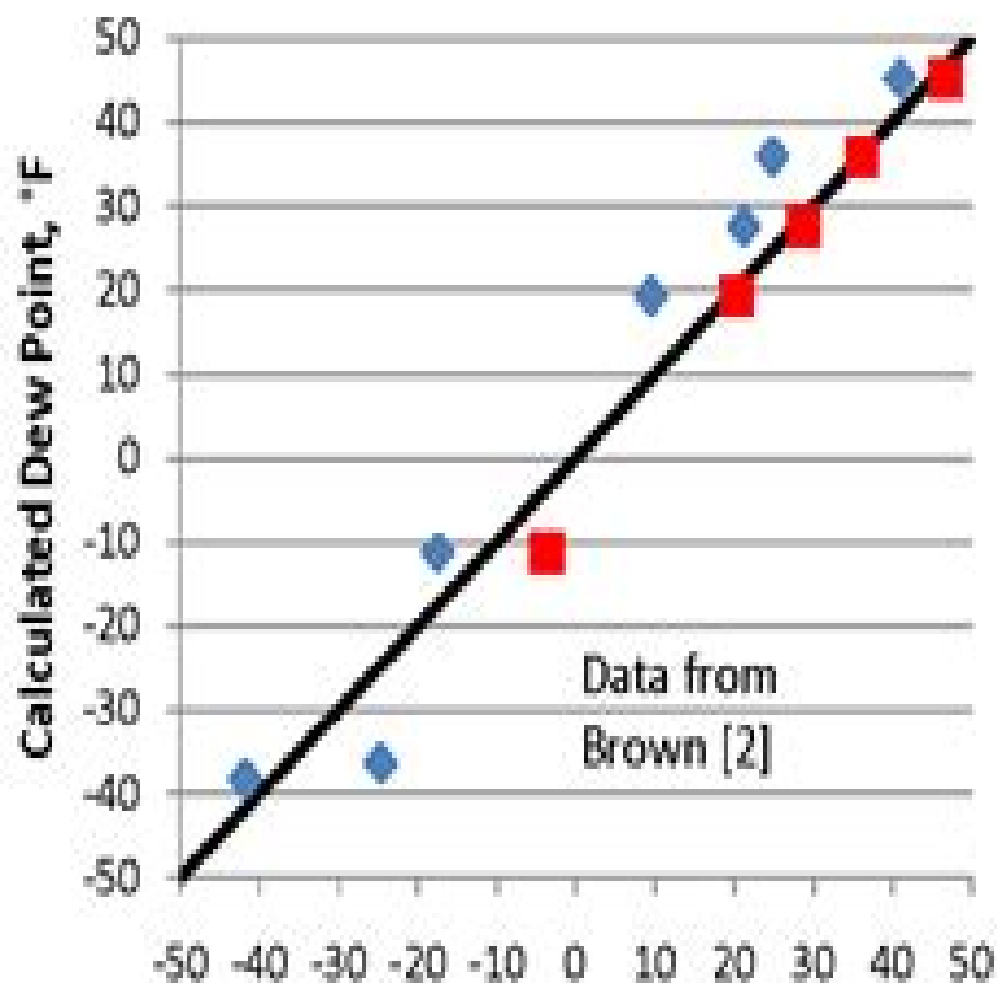
Figure 3 NPL Natural Gas Dew Points Manual & Automated Chilled Mirror vs. ProMax PR
