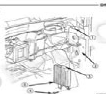
Fig. 11 Power Amplifier Removed/Installed
