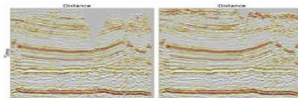
Figure 1. Prestack time migration for a land data set in the Marcellus area without (left) and with (right) 5D interpolation.
