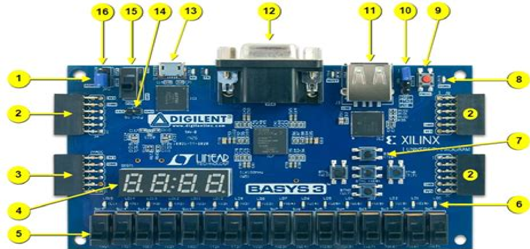
Figure 1. Basys 3 FPGA board with callouts.
