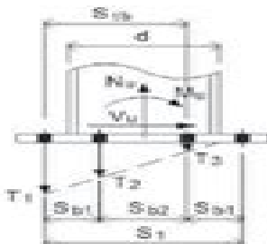
4 BOLT LINE
