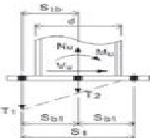
3 BOLT LINE
