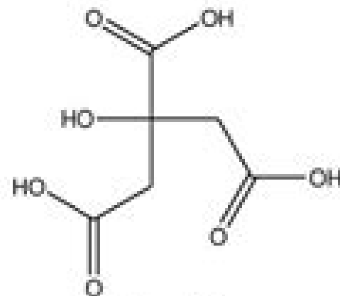
citric acid (oranges, TCA cycle)
