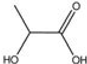
lactic acid 2-hydroxypropanoic acid (causes muscle cramps due to O 2 debt)
