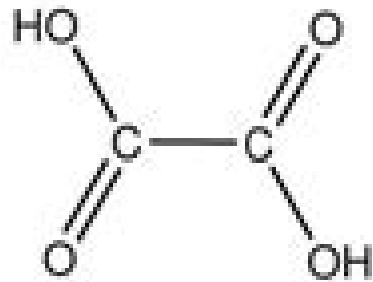
oxalic acid ethandioic acid (poison in rhubarb leaves)
