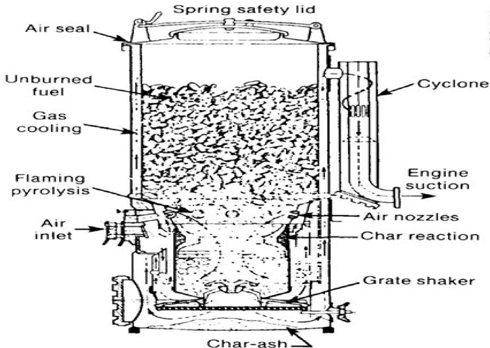
Fig. 5-2. Imbert (nozzle and constricted hearth) gasifier (Source: Gengas 1950, Fig. 75)
