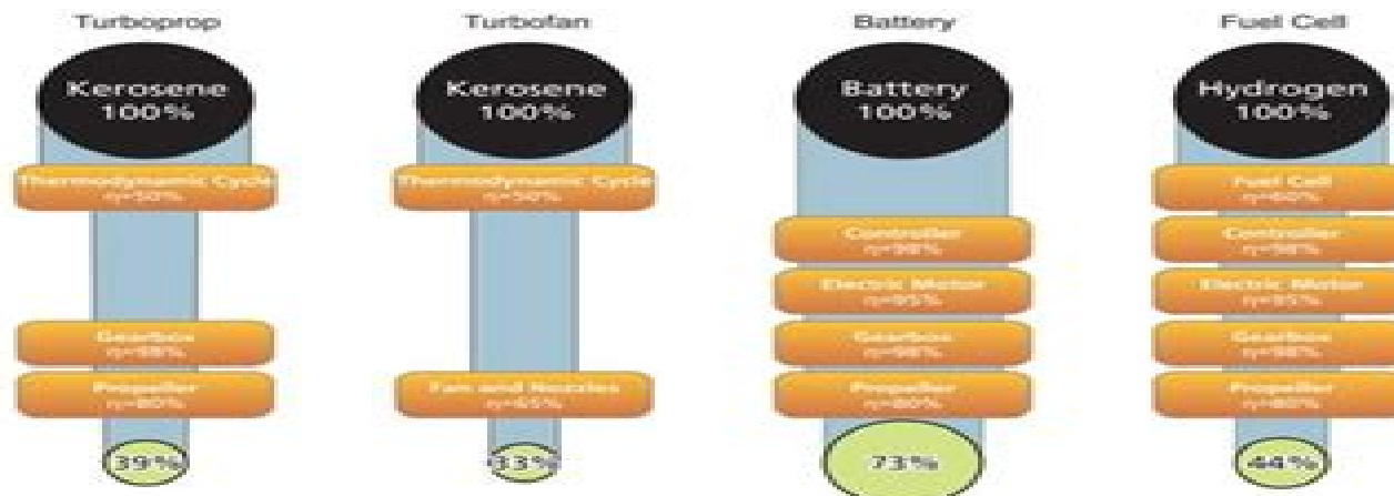
Figure 7 Typical on-board conversion chains with typical component efficiencies and total chain efficiency.
