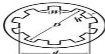
Fig. 7c. 10-Spline Fitting
