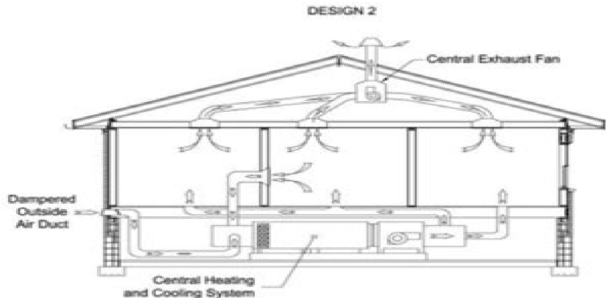
Figure 7-14 Whole House Ventilation System
