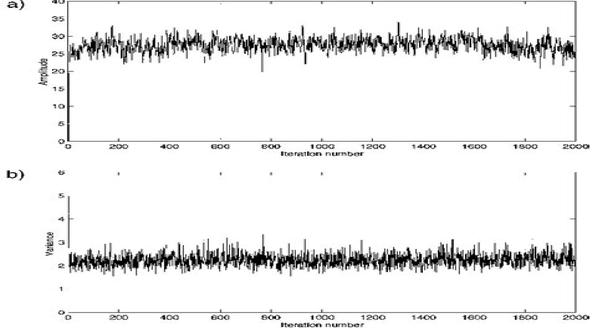
FIG. 3. Monitoring maximum wavelet amplitude (a) and seismic noise variance (b).
