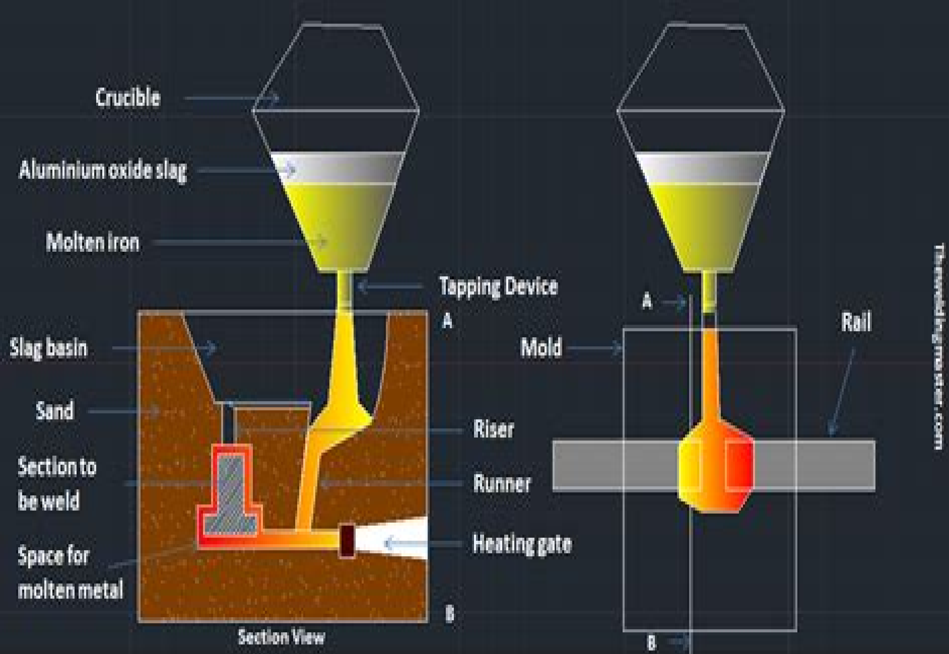
Thermit Welding Process
