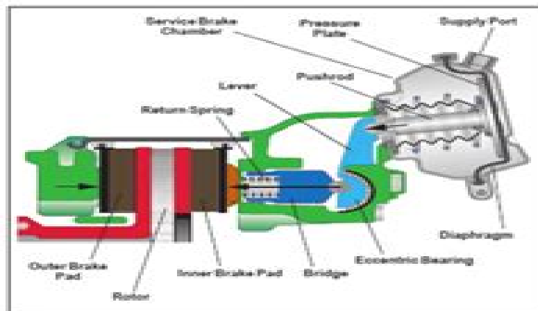
FIGURE 2 - CROSS-SECTION VIEW SHOWING BRAKE OPERATION
