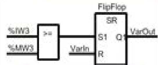
Function Block Diagram
