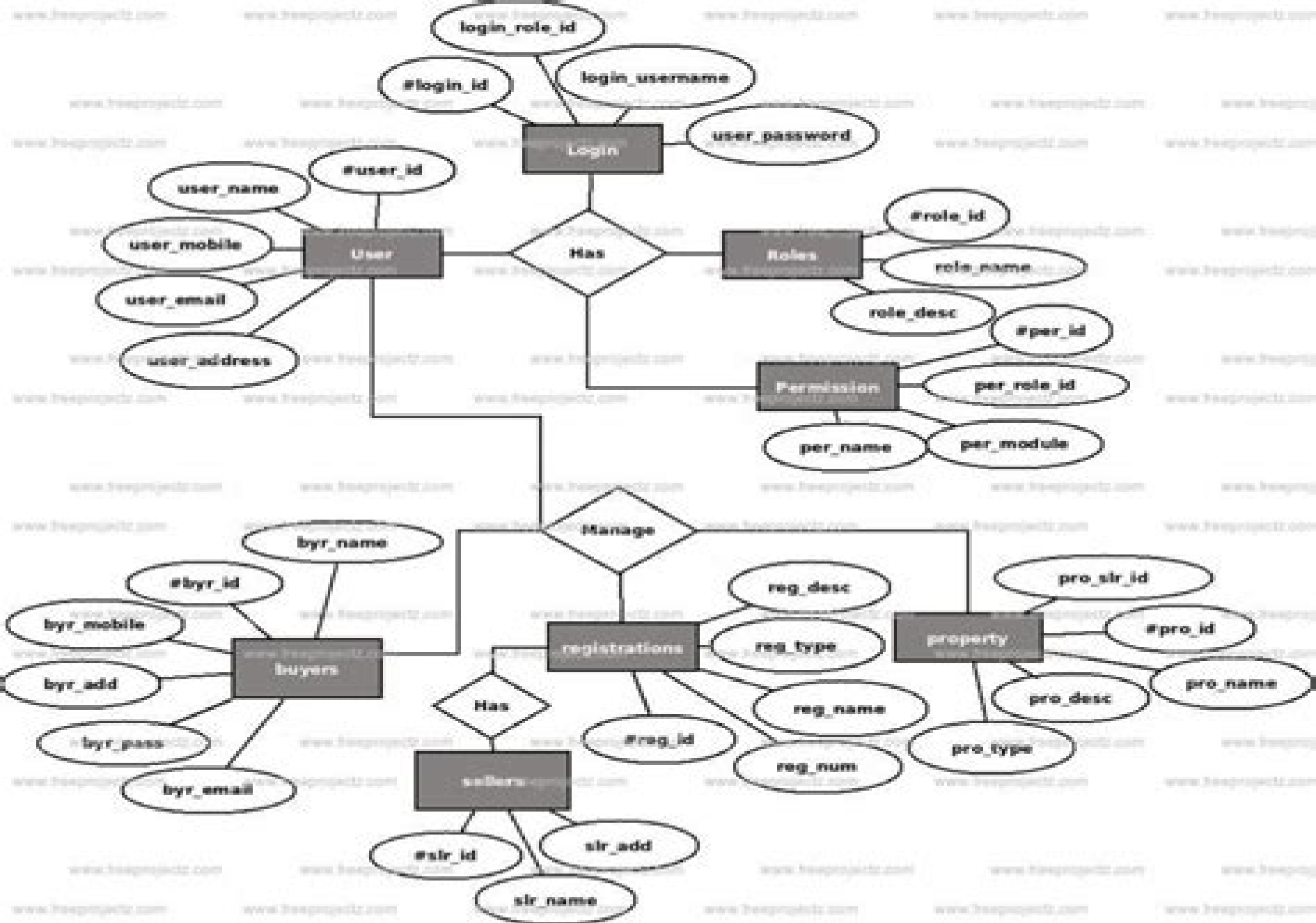
ER Diagram For Property Management System
