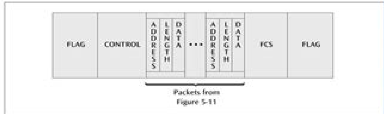
Figure 5-12 Frame layout for the information packet transferred between statistical multiplexors
