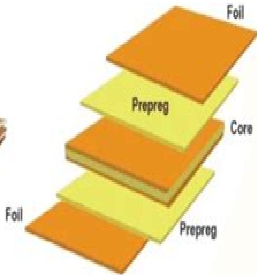
PCB Prepreg
