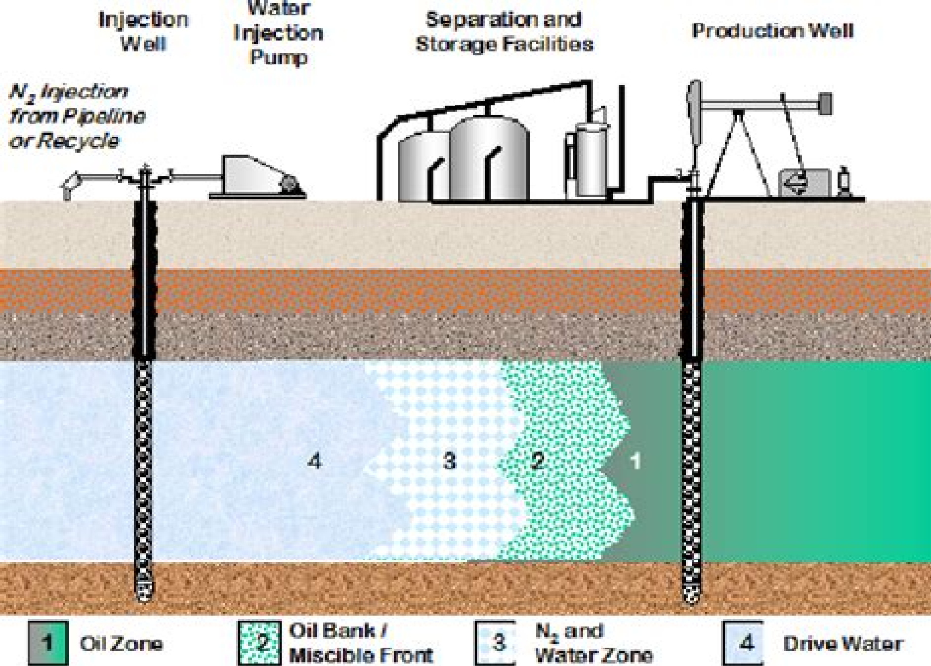
Fig. 4. Nitrogen miscible displacement.
