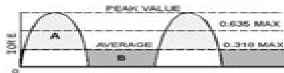
Figure 2.1 half- and full-wave rectified signal
