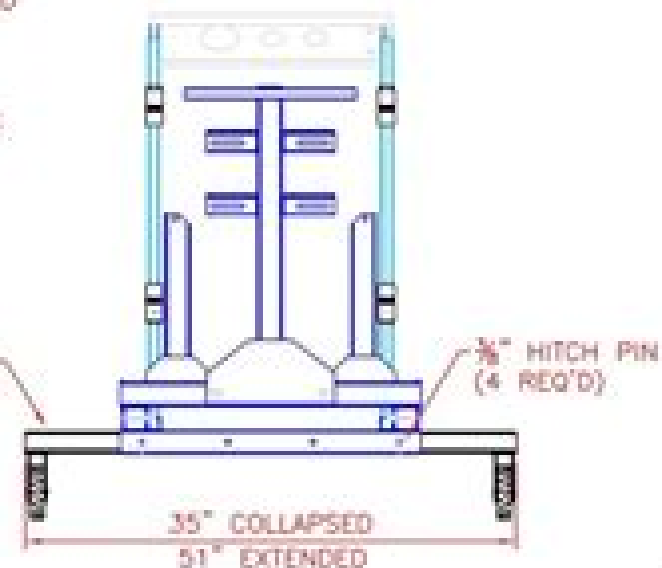
ASSEMBLY
