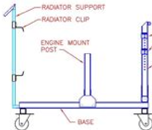
ENGINE STAND
