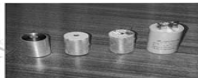
Fig.1: From left: the coiled cylindrical element; the element with the sprayed ends; the element with the two connection wires; and the complete capacitor.
