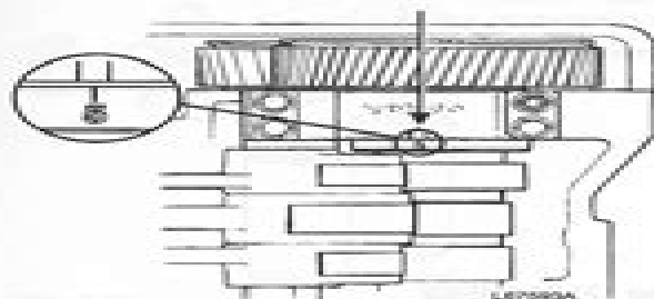
Fig. 146 Cam shaft marking
