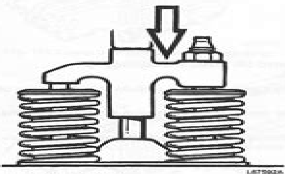
Fig. 148 Valve yoke
