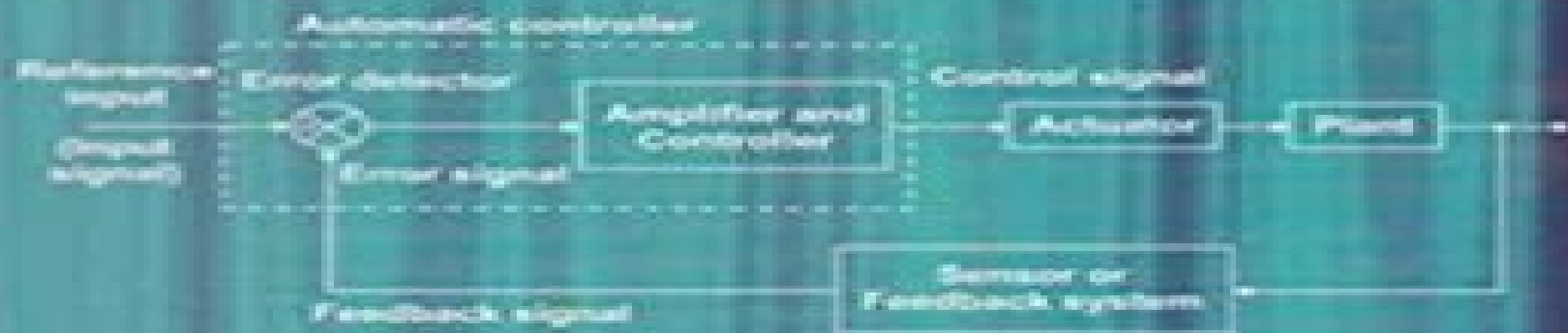
Block diagram of automatic control system
