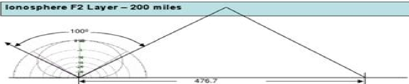
Figure 1: Required NVIS Antenna Vertical Directivity Pattern
