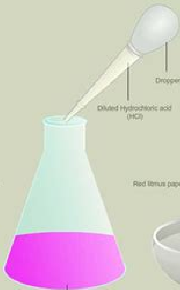
Sodiumhydroxide + Phenolphthalein
