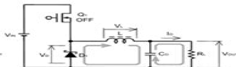
Fig. 2: Basic Buck Converter Circuit Switching Element OFF
