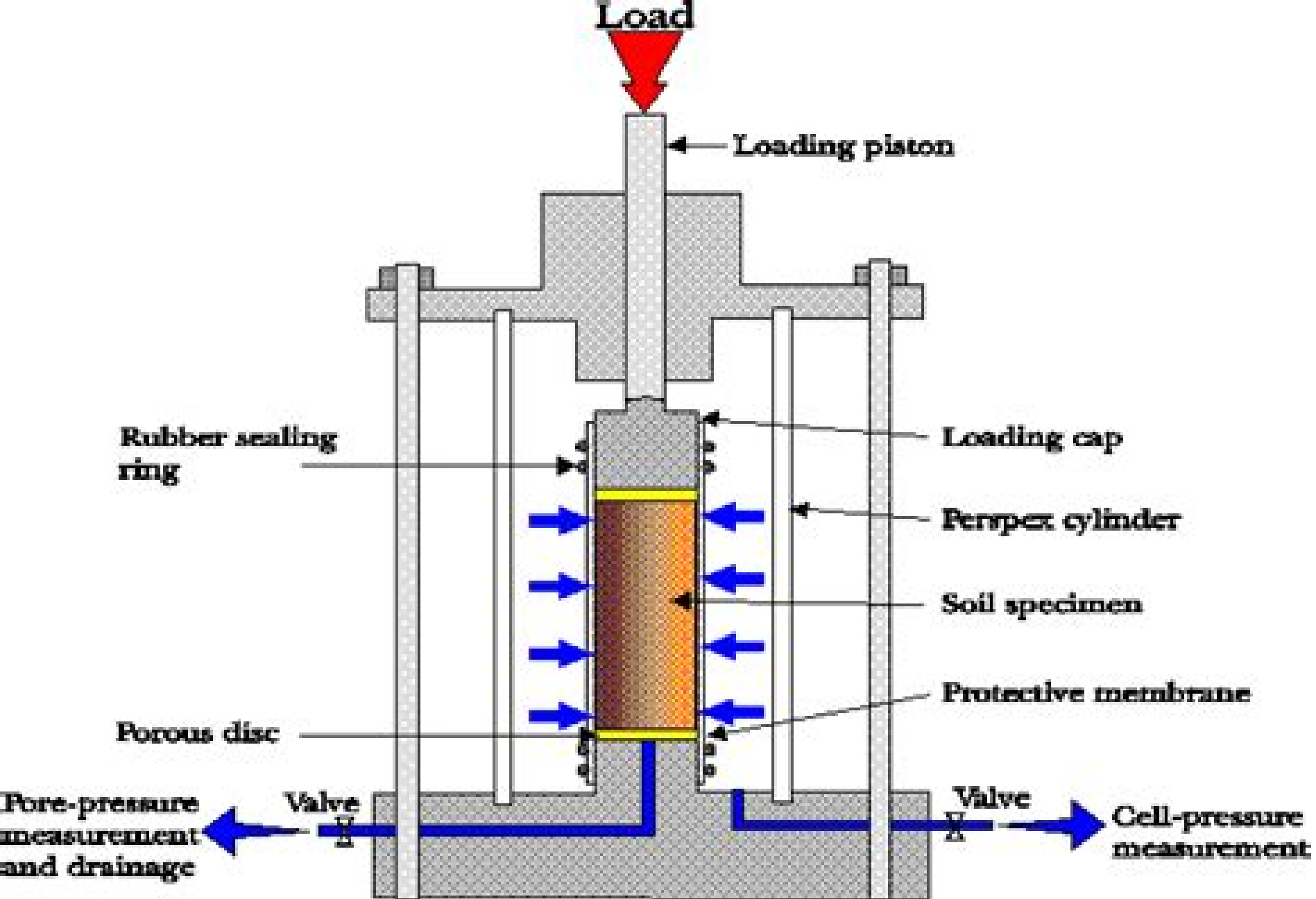
Triaxial apparatus
